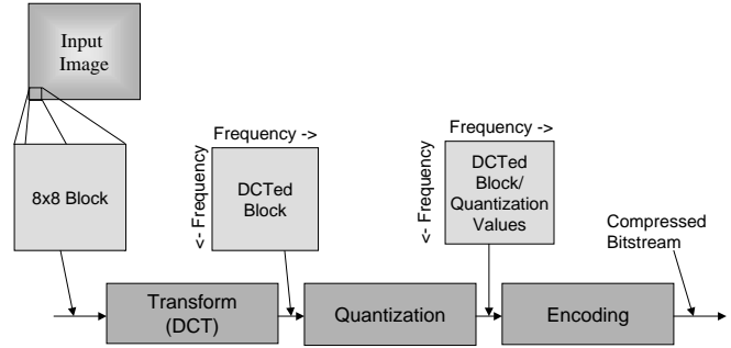
Fig. 2. Basic flow of JPEG image compression algorithm
