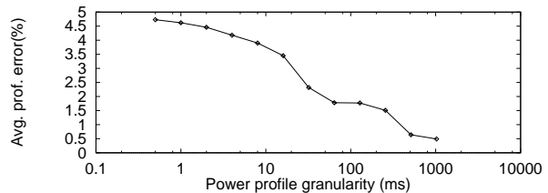
Figure 7: Effect of granularity on average profiling error
